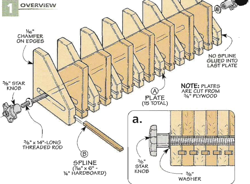
▲ V-Block. The V-block makes it easy to drill a hole in a dowel or round stock. The individual plates of the V-block can be adjusted for different diameters.
