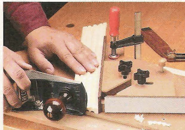
▲ Other Angles. By disengaging the locking pin and securing the stop block with a clamp, you can use the shooting board to trim miters at any angle.
