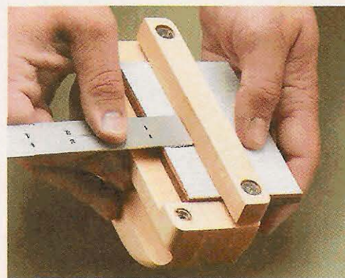
▲ Setup. Now adjust the sanding pad to match the width of the edging. Then tighten the screws to lock the fence in place.
