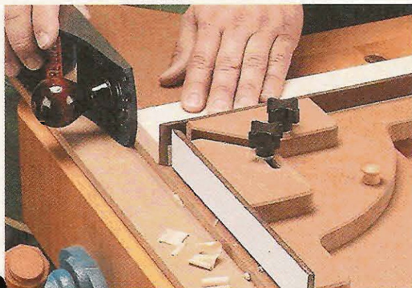
▲ Shooting End Grain. With the stop block set perpendicular to the edge of the shooting board, you can shave a hair off the end of a workpiece.
