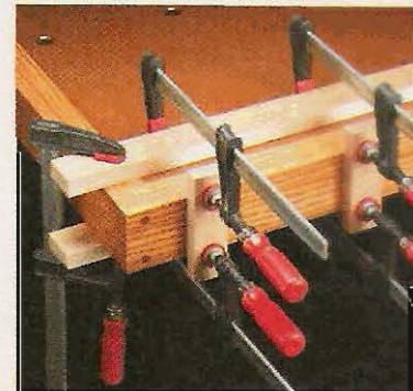
▲ "Stretching" Your Clamps. A couple of cleats attached to the top of the bench allow you to clamp the end apron in place.
