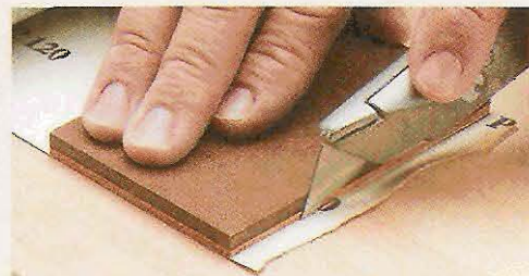
▲ Size the Sandpaper. After sticking an oversized piece of sandpaper to the pad, use a utility knife to trim the edges flush.
