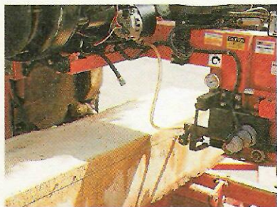
10 To prevent pitch from gumming up the blade, a water-drip system keeps it running cool.
