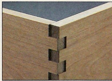
Short Pins. If the router bit is set too shallow, you'll end up with pins that are too short.
