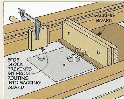
Step 3: Stop Block. Position a stop block on the fence to prevent the bit from cutting through backing board.
