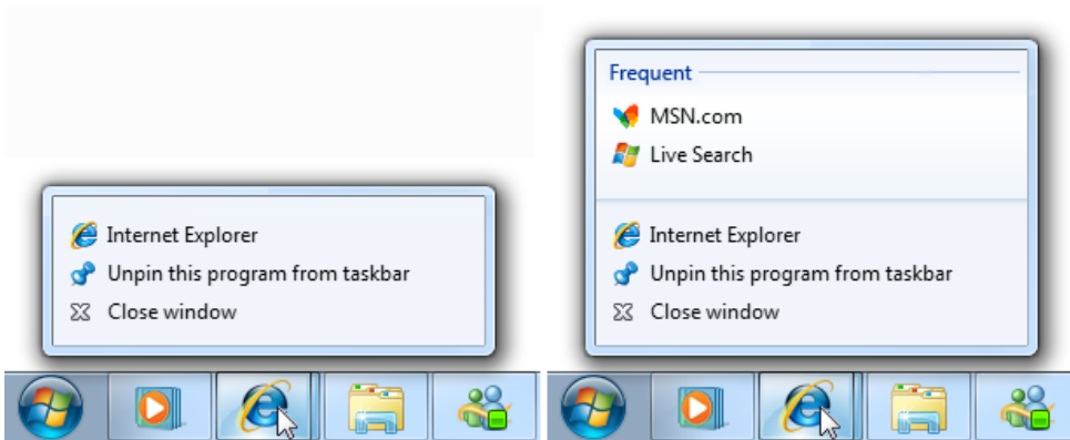
In this example, a taskbar Jump List immediately displays the standard items, and then slides out to display the destinations once the list is ready. Doing so disguises the time required to build the list. By contrast, delaying the initial display would feel unresponsive, and displaying an incomplete list or progress feedback would feel much slower.
