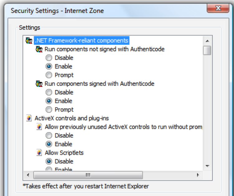
In this example, the tree leaves are options and the containers are option categories.
